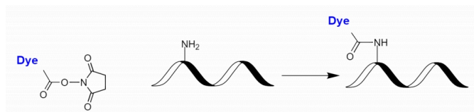
Figure 1. Fluorescent dye NHS esters (or succinimidyl esters) are the most popular tool for conjugating dyes to a peptide, protein, antibody, amino-modified oligonucleotide, or nucleic acid. NHS esters react readily with the primary amines (R-NH 2 ) of proteins, amine-modified oligonucleotides, and other amine-containing molecules. The resulting dye conjugates are quite stable.
